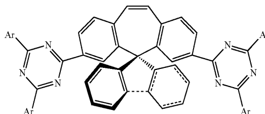
chemical formula 5
