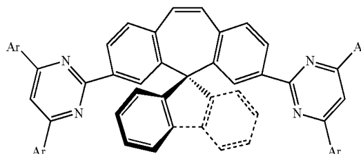
chemical formula 3
