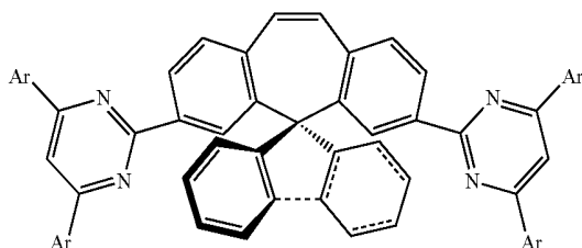
chemical formula 3
